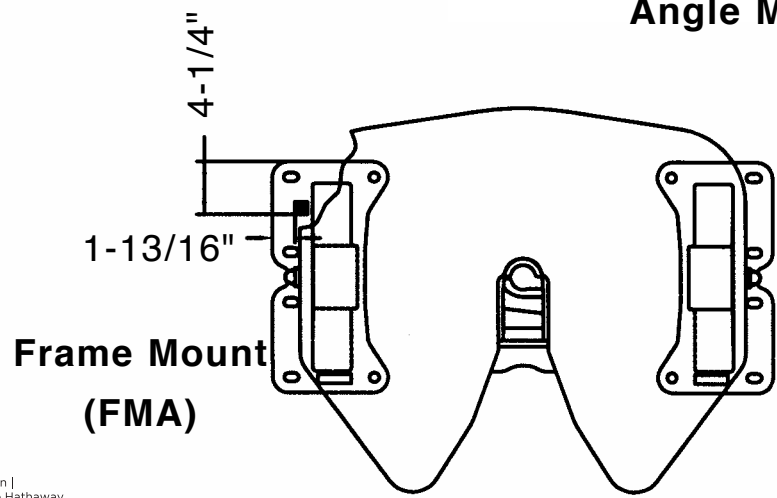
D3 Frame Mount
