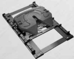
H7 AWX HD Slide 70,000 lbs vertical load 200,000 lbs drivebar pull
