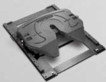
H7 AWB Slide 62,500 lbs vertical load 150,000 lbs drivebar pull
